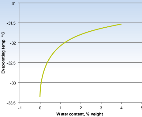
R717 Evaporating temperature shift due to water content at 1 atm.
